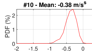
PC to Fuselage Out Deceleration (ms 2 )
